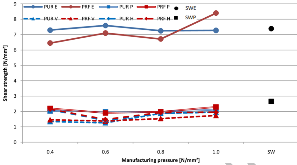
Figure 5. 5-percentile shear strength values for different test configurations
