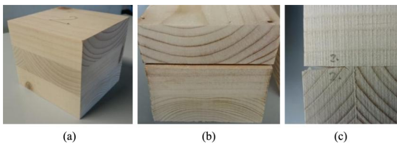
Figure 8. Specimen for delamination test before (a) and after vacuum-pressure cycle (b, c)
