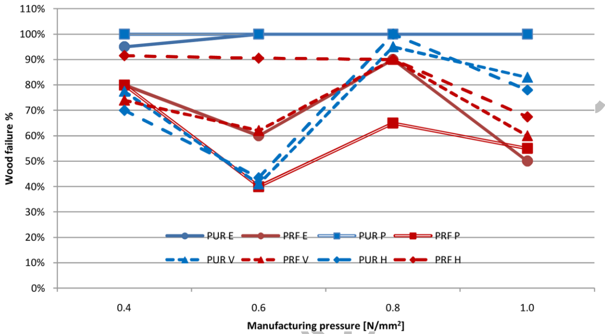
Figure 6. Median wood failure percentage values for different configurations of specimens manufactured with different pressures
