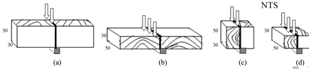
Figure 2. Shear test specimens for: end-grain (a), perpendicular to grain (b) loading, and crosslam bonded elements vertically (c) and horizontally (d) loaded (dimensions in mm)
