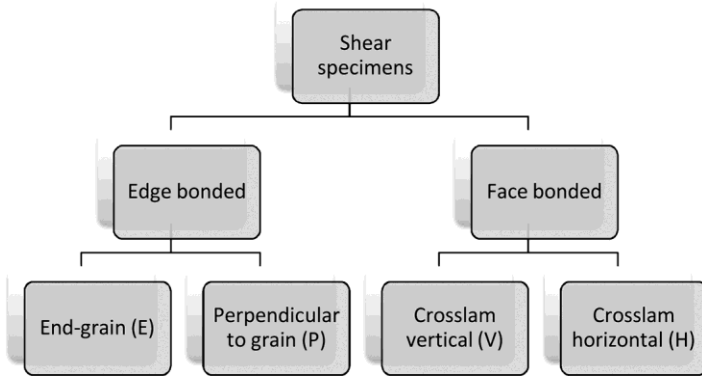
Figure 1. Schema of specimen configurations for shear tests
