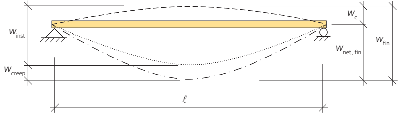
Figure 9.1 Definitions of deflection
