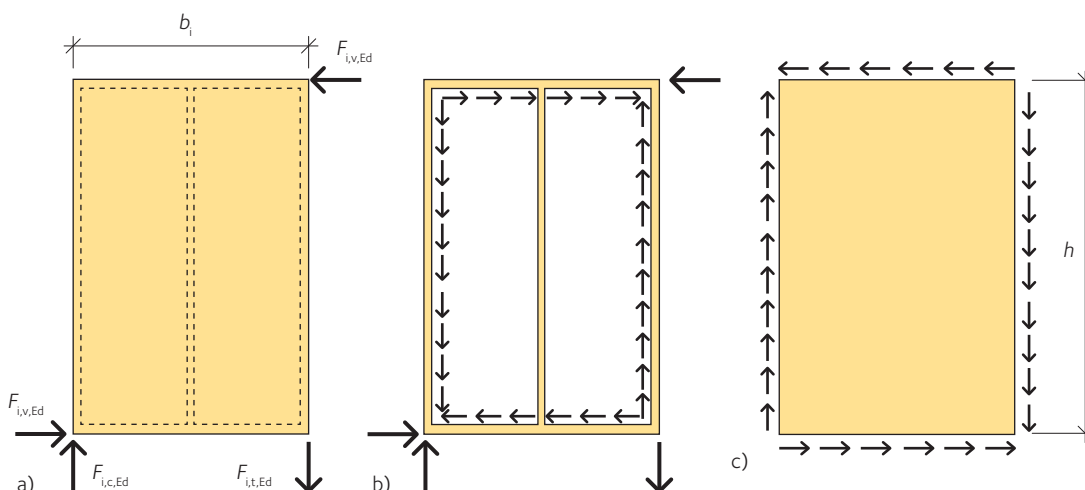
Figure 11.1 Forces acting on a) wall panel; b) framing; c) sheathing in wall diaphragm.
