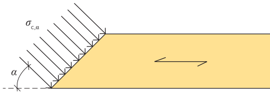
Figure 7.1 Compressive stresses at an angle to the grain
