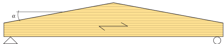
Figure 8.1 Double tapered beam
