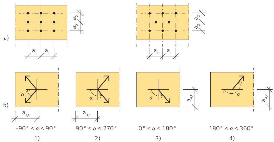
Figure 10.4 Definition of edge and end distances and spacings between fasteners
