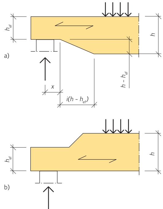
Figure 8.3 End-notched beams
