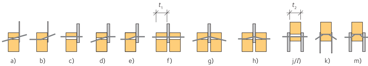
Figure 10.2 Failure modes for steel-to-timber connections. The letters refer to the respective design expression above.
