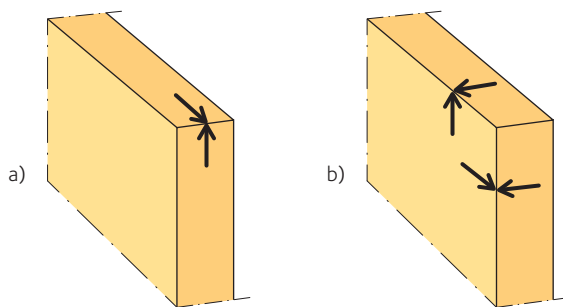
Figure 3.2 Definition of a) panel shear and b) planar shear.
