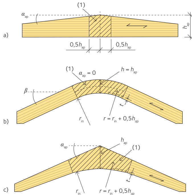
Figure 8.2 a) Double tapered, b) curved and c) pitched cambered beams. Fibre direction parallel to the lower edge. The part marked (1) in the figure is the stressed/curved volume V .
