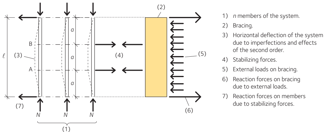
Figure 12.2 Beam or truss system supported by lateral bracing
