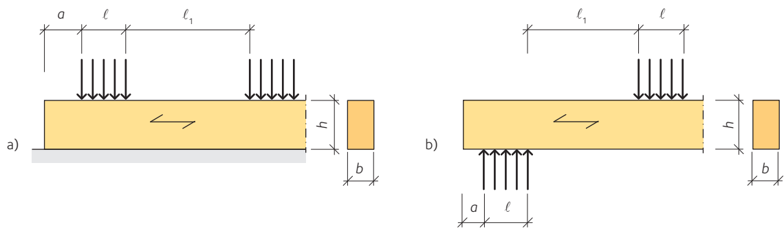
Figure 5.1 Member on a) continuous supports (for example a ground plate on a concrete slab) and b) discrete supports (for example a beam supported by columns).
