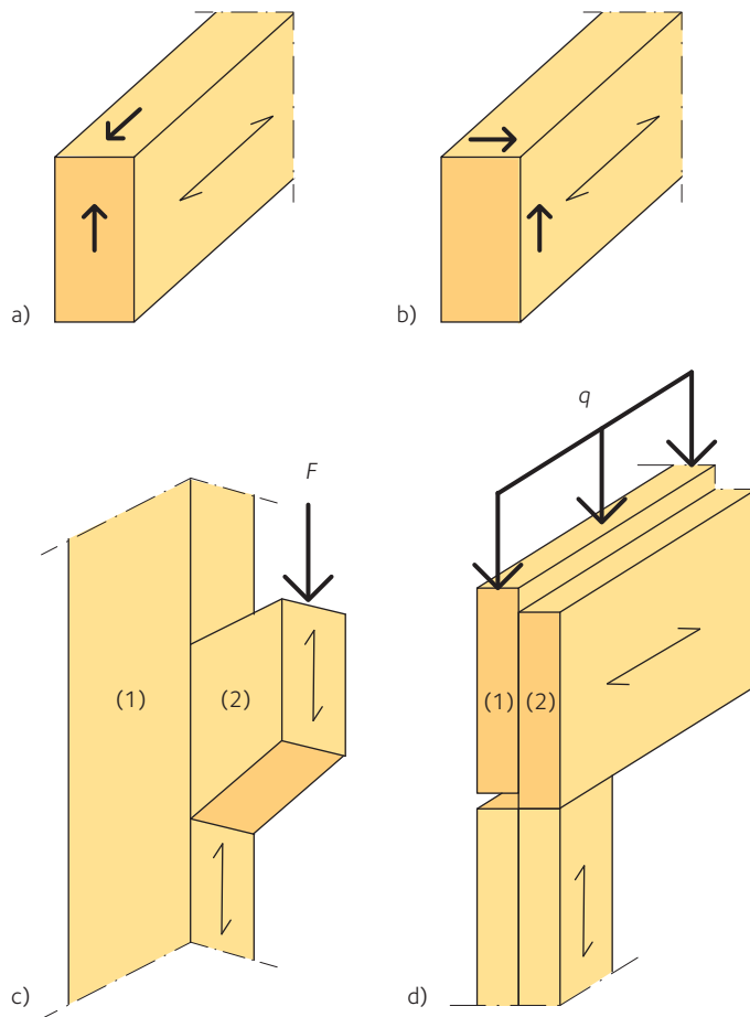
Figure 3.1 a) Member with a shear stress component perpendicular to grain (shear). b) Member with both shear stress components perpendicular to grain (rolling shear). Two practical examples. c) Glued wooden cleat on column, shear between contact surfaces (1) and (2). d) Two beams glued together, rolling shear between contact surfaces (1) and (2).
