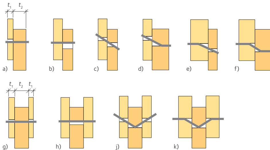
Figure 10.1 Failure modes for timber and panel connections
