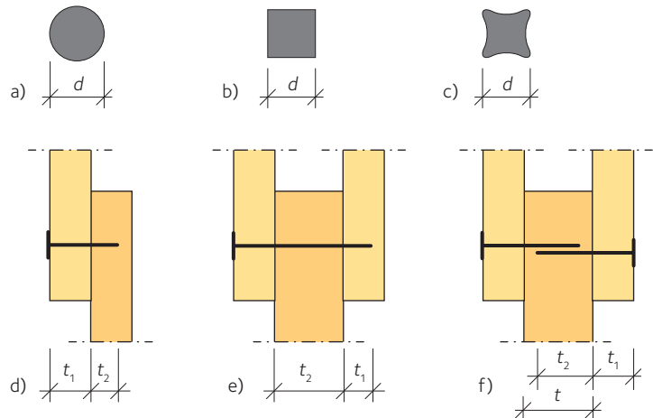
Figure 10.3 Nominal diameter d for a) round, b) square and c) grooved nail. Definition of t_1 and t_2 for d) single shear connection, e) double shear connection and f) overlapping nails.
