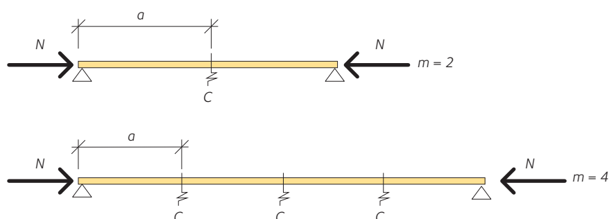
Figure 12.1 Single members in compression braced by lateral supports (C)
