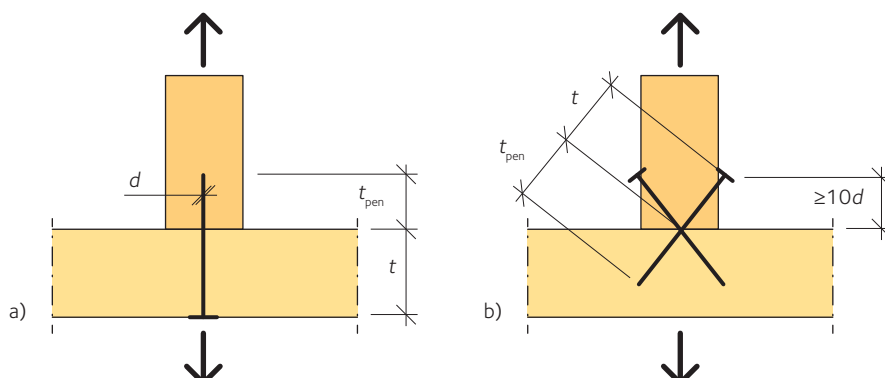
Figure 10.5 Nailing a) perpendicular to grain and b) slant nailing.
