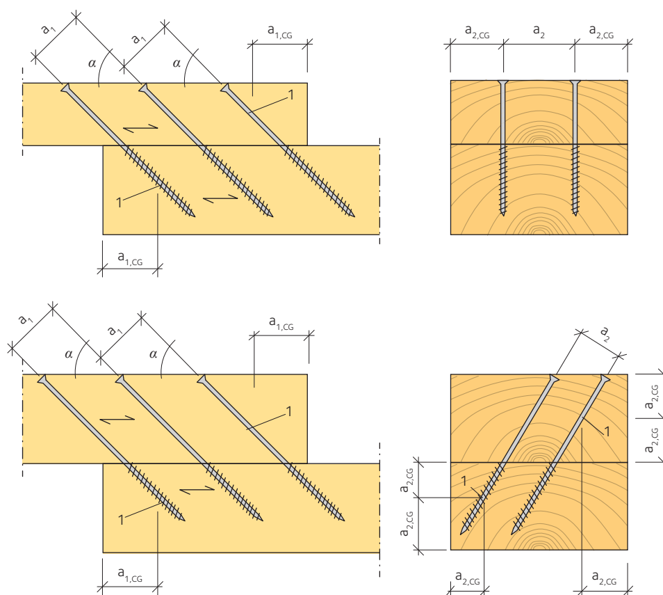
Figure 10.6 Spacing and end/edge distances for axially loaded screw connections
