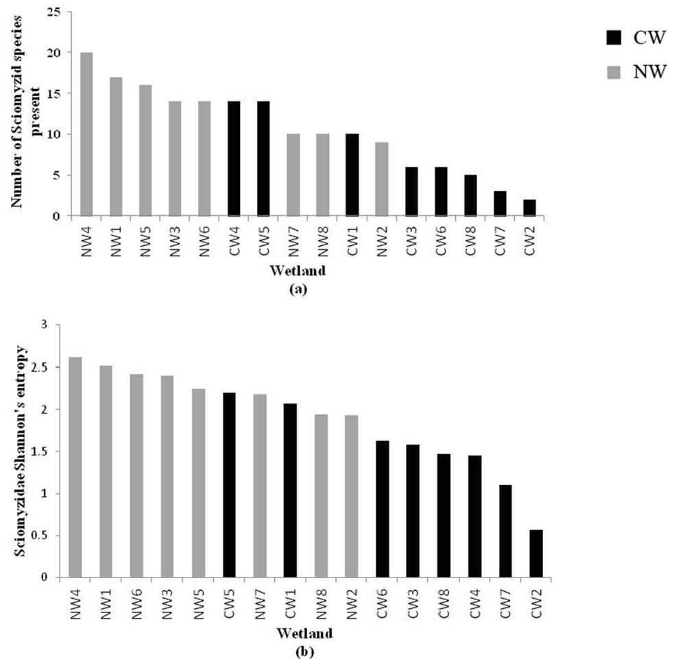
Fig. 4 a Sciomyzidae species richness; b Shannon's entropy at CWs and NWs
